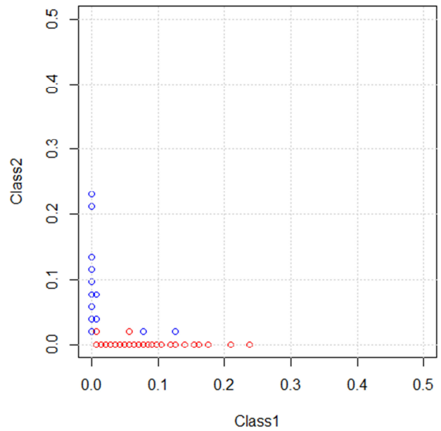
DD-Plot (random Tukey) for ecoli_cpvspp
