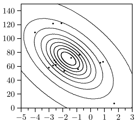
(c) Mahalanobis depth ( \alpha = 0.1, 0.2, 0.3, 0.4, 0.5, 0.6, 0.7, 0.8, 0.9 )
