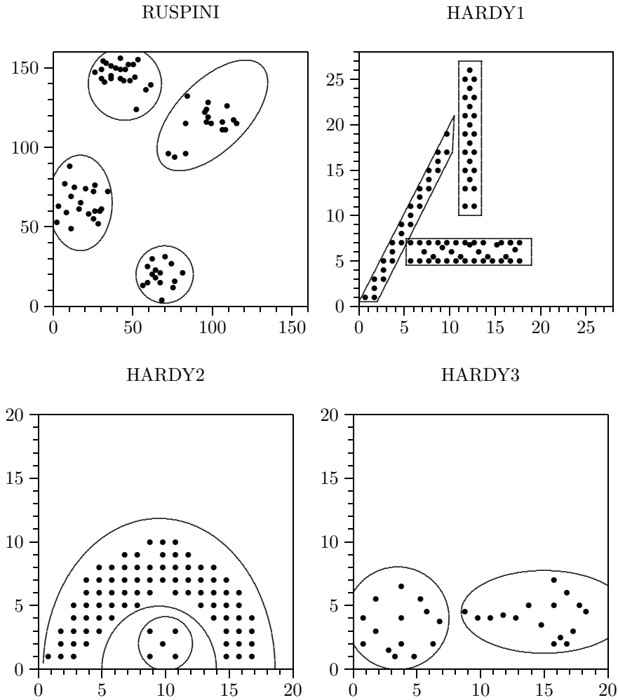
FIGURE 2. Four artificial data sets with given classes.
