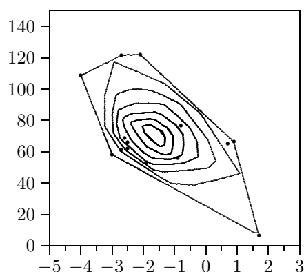
(a) zonoid depth ( \alpha = 1/15, 3/15, 5/15, 7/15, 9/15, 11/15, 13/15 )
