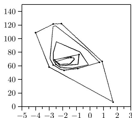
(b) halfspace depth ( \alpha = 1/15, 2/15, 3/15, 4/15, 5/15 )
